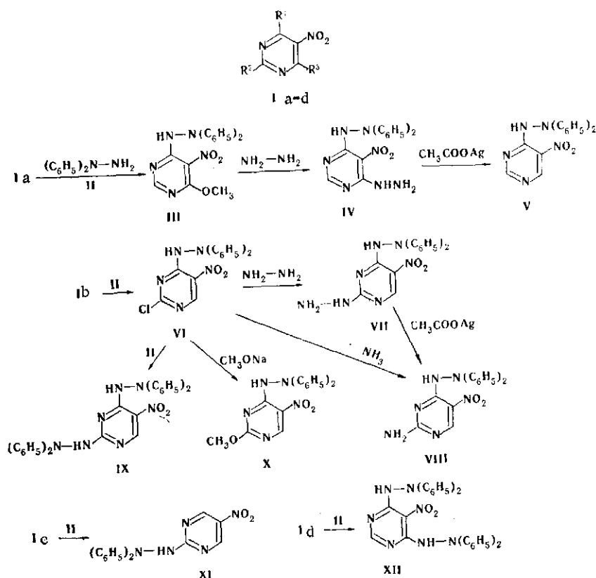
Ia R 1 =Cl, R 2 =H, R 3 =OCH 3 ; b R 1 =R 2 =Cl, R 3 =H; c R 1 =R 3 =H, R 2 =Cl; d R 1 =R 3 =Cl, R 2 =H
