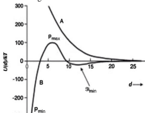
Fig. 1 Theoretical interaction potential between a pair of spherical emulsion droplets.
