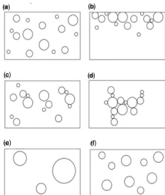
Fig. 2 Schematic representation of the key mechanisms of O/W emulsion instability: (a) stable dispersion of droplets; (b) creaming; (c) flocculation (weak); (d) flocculation (strong); (e) coalescence; (f) Ostwald ripening.
