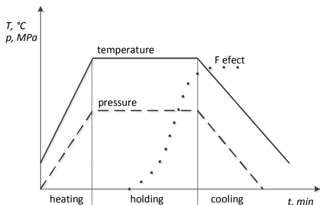
Fig. 2. Time-temperature diagram of work process
