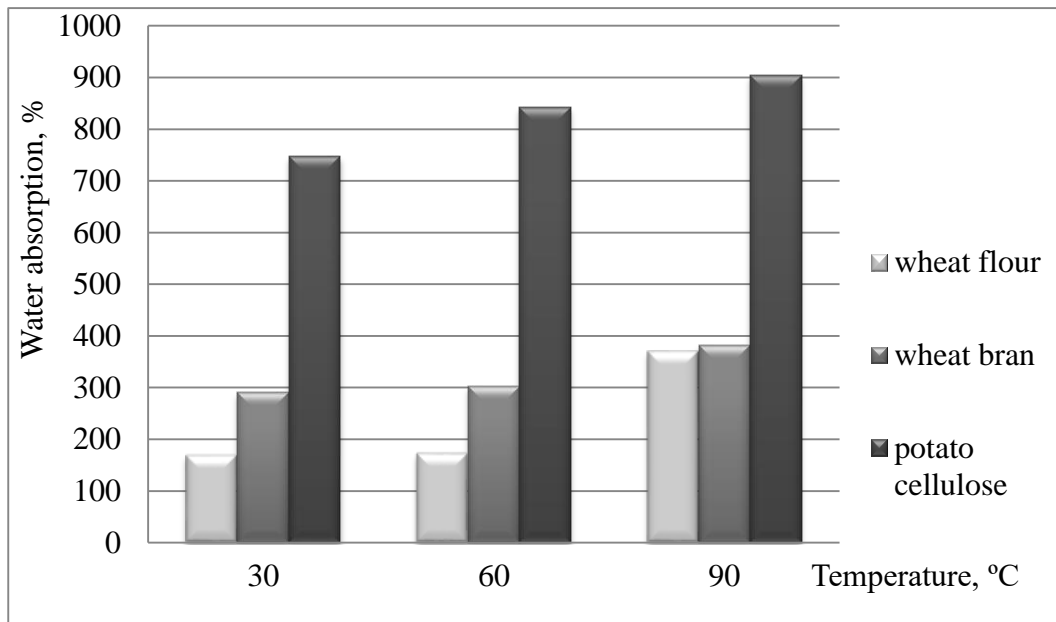
Figure 1. Water absorption of potato cellulose
