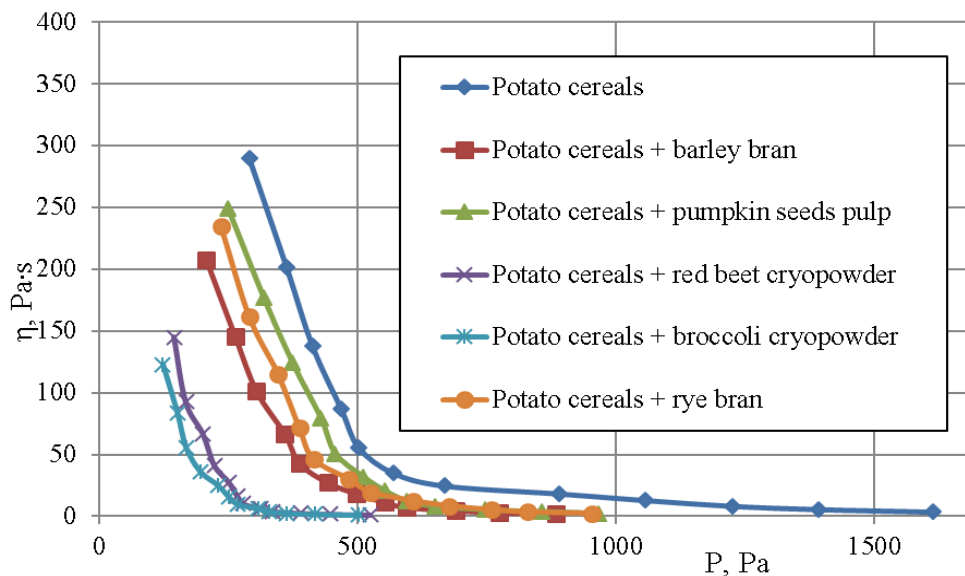
Fig. 3 Curves of viscosity of model solutions of samples of semi-finished products of FPC
