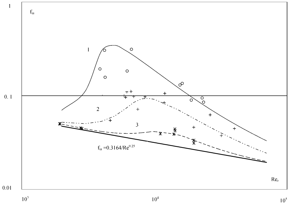
Рис. 5. Залежність f_{ia} від Re_p : 1- Re_p -1000, We =4500; 2- Re_p -700, We =5000; 3- Re_p -400, We =5500; \circ - Re = 800-1200, We = 4000-5000; + - Re = 600-800, We = 4500-5500; * - Re = 300-500, We = 5000-6000.
