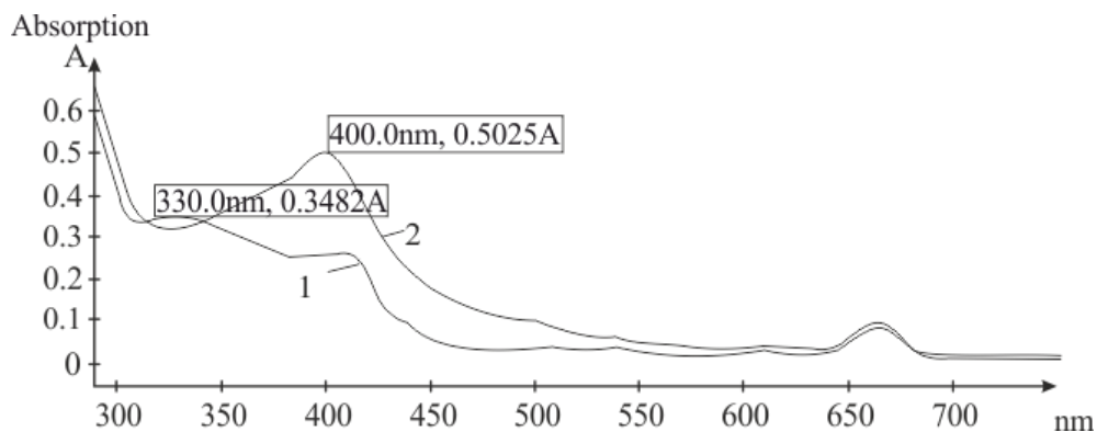
Figure 3. Electronic absorption spectrum of ethylacetate extracts after hydrolysis of leaf extracts (1-pH=6,5; 2-pH=11,8)
