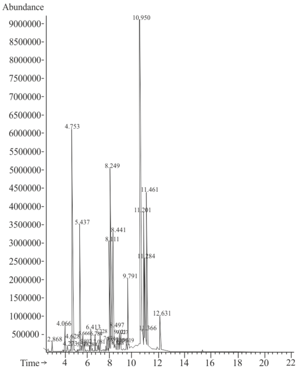
Figure 7. Mass-chromatogramm of TMS derivates of initial ethanol extracts of fenugreek leaf
