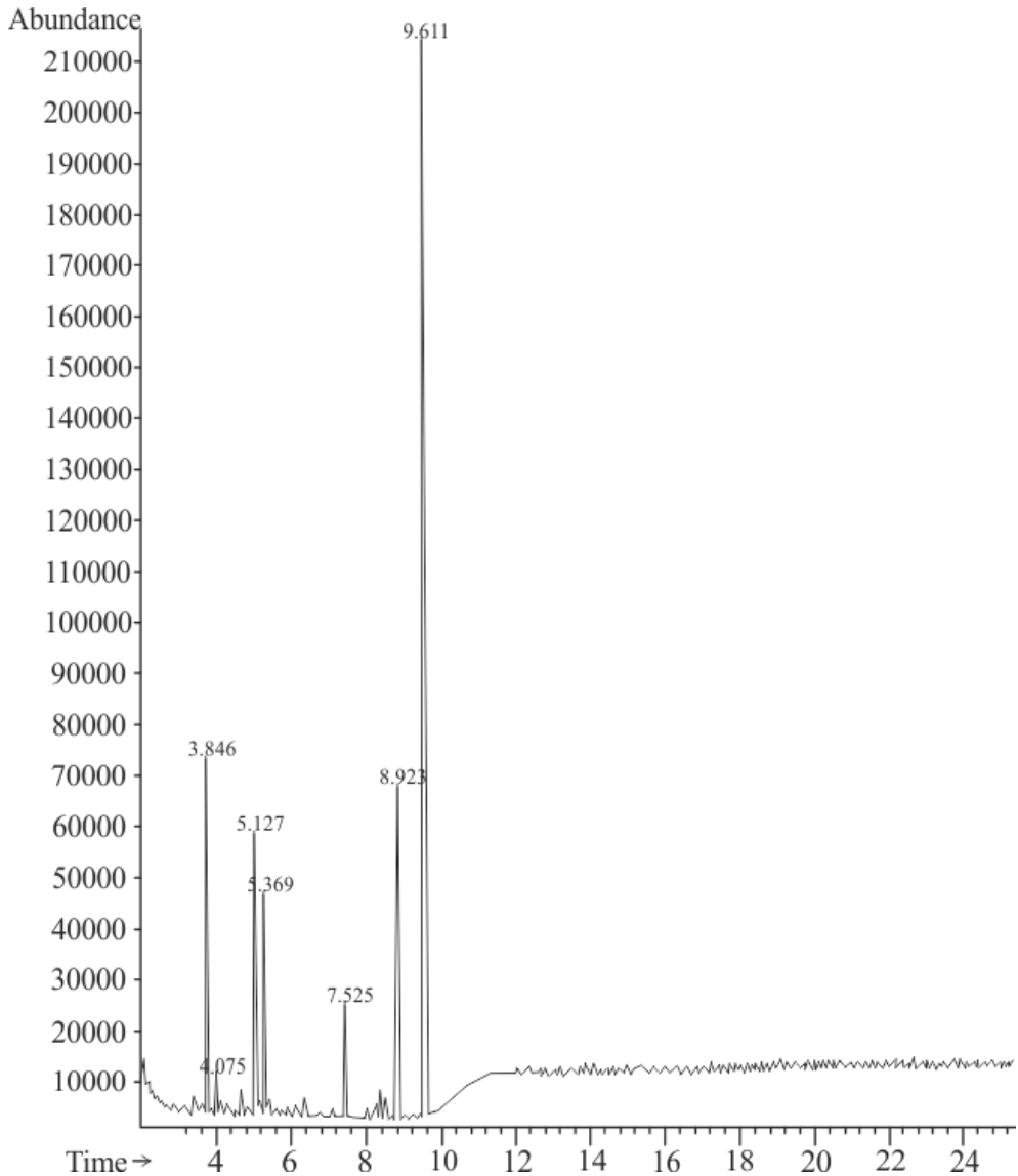
Figure 6. Mass-chromatogram of ethylacetate extracts after hydrolysis of fenugreek leaf extracts
