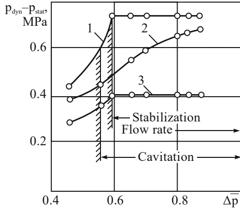
Fig. 9. Dependence of the difference between the dynamic and static flow pressure on the pressure drop across the cylindrical throttle: 1 – compressed cross-section; 2 – initial cross-section; 3 – inlet cross-section
