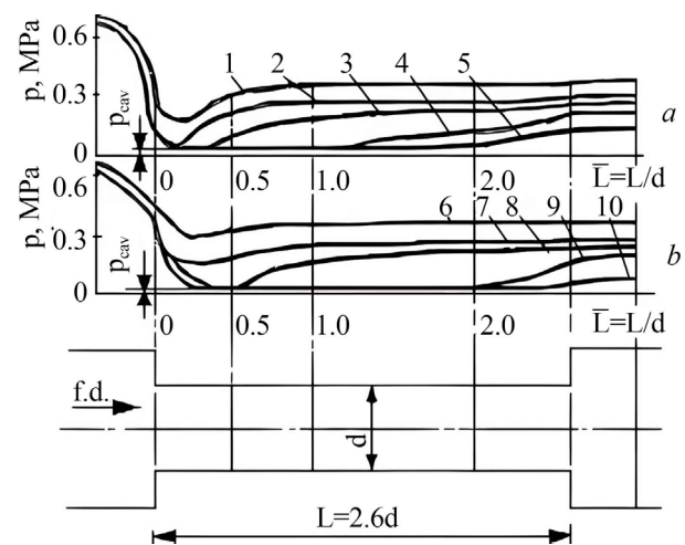
Fig. 8. Distribution of static pressure along the flow length in a cylindrical throttle: a – in the near-wall region; b – along the axis of the channel; 1, 6 – \Delta\bar{p}=0.47 ; 2, 7 – \Delta\bar{p}=0.56 ; 3, 8 – \Delta\bar{p}=0.59 ; 4, 9 – \Delta\bar{p}=0.65 ; 5, 10 – \Delta\bar{p}=0.84
