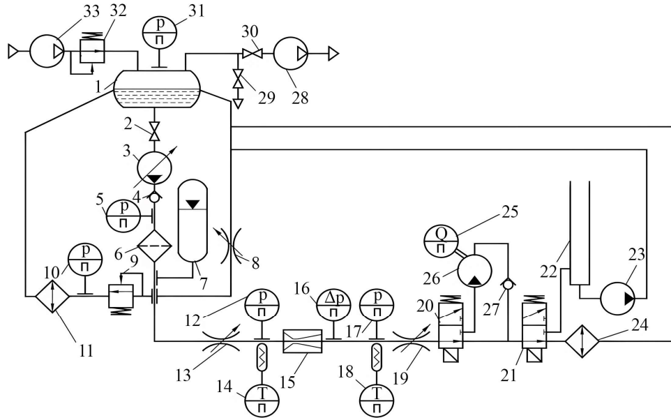
Fig. 1. Basic hydraulic scheme of the experimental bench for the study of cavitation effects: 1 – hydraulic tank; 2, 29, 30 – shut-off valves; 3 – volumetric pump; 4, 27 – check valves; 5, 10, 12, 17, 31 – manometers; 6 – filter; 7 – hydraulic accumulator; 8, 13, 19 – throttle valves; 9 – safety valve; 11, 24 – heat exchangers; 14, 18 – thermometers; 15 – cavitation generator; 16 – pressure pulsation sensor; 20, 21 – electromagnetic taps; 22 – measuring tank; 23 – centrifugal pump, 25 – flow meter sensor, 26 – flow meter, 28 – vacuum pump, 32 – reducer; 33 – compressor
