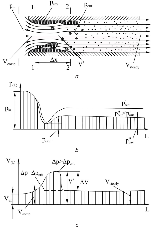
Fig. 10. Cavitation outflow of liquid through a cylindrical throttle: a – distortion of flow lines and generation of caverns; b – pressure change in the flow; c – change in flow rate
