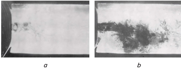
Fig. 6. Caverns in the drain line behind the throttle: a – \Delta\bar{p}=0.78 ; b – \Delta\bar{p}=0.88
