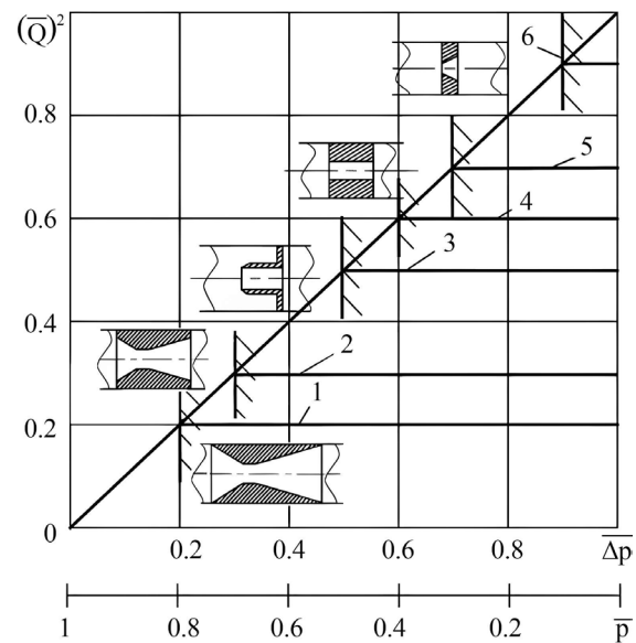
Fig. 11. Flow rate and drop characteristics (\bar{Q})^2 = f(\bar{p}, \Delta\bar{p}) of throttle devices (working fluid AMG-10): 1 – nozzle of the confusor-diffuser type; 2 – nozzle of the confusor-diffuser type, shortened; 3 – Bord nozzle; 4 – cylindrical nozzle; 5 – nozzle with a rectangular channel; 6 – diaphragm
