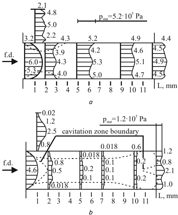
Fig. 7. Diagrams of distribution of static pressure in the intersections of a choke with a rectangular channel: a – \Delta\bar{p}=0.58 ; b – \Delta\bar{p}=0.81
