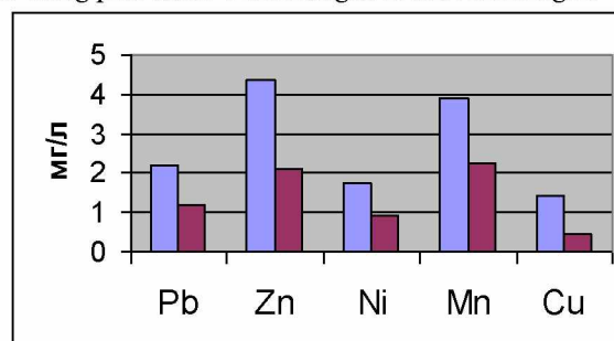
Fig. 1 Content of heavy metals in table beet juice, processed with shungite in comparison with the control sample
