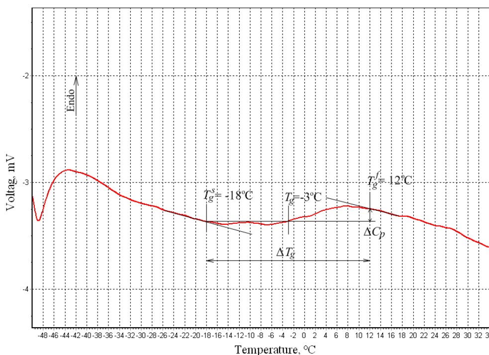
Fig. 1 Typical DSC heating curve for whey powder showing the glass transition
